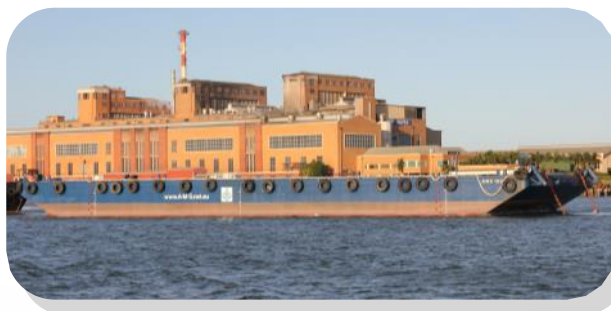
A.M.S. 1803 180ft x 70ft x 14ft Deck Cargo Ballast Tank Barge
